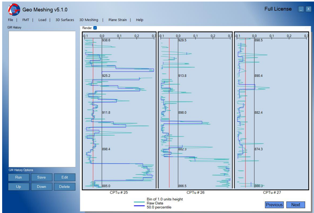
Figure 15: State Parameter Statistical Analysis.
