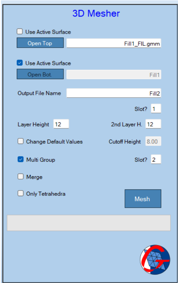
Figure 69: 3D Meshing Window – Fill2 3D Model.
